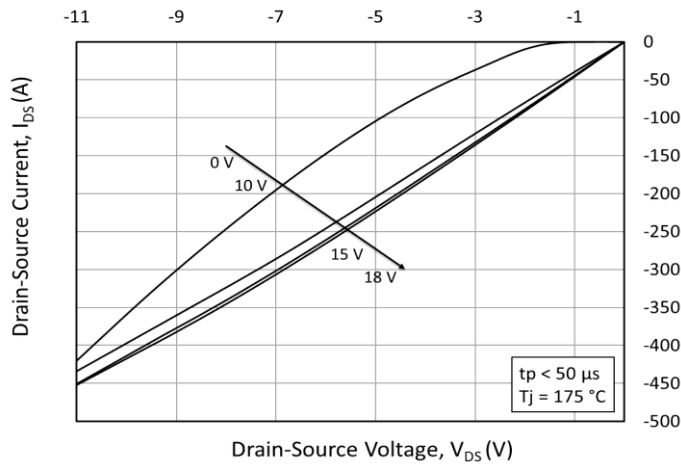
Figure 15. 3rd Quadrant Characteristic at T_{VJ} = 175\text{ °C}
