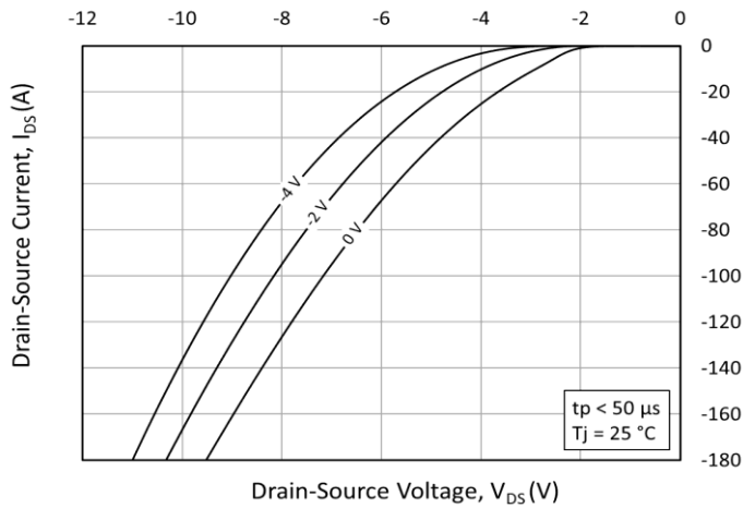
Figure 9. Body Diode Characteristic at T_W = 25^\circ\text{C}
