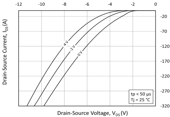
Figure 9. Body Diode Characteristic at T_{VJ} = 25\text{ }^\circ\text{C}
