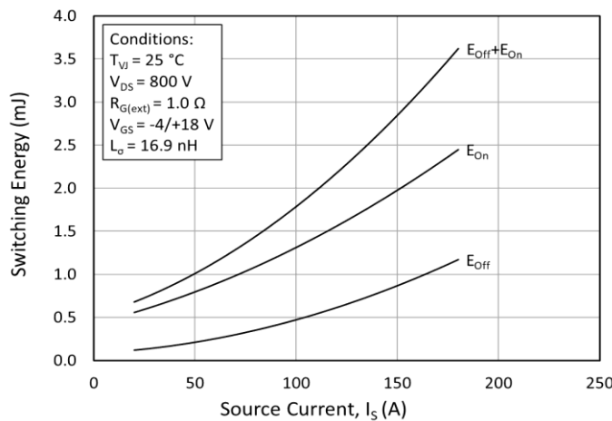
Figure 23. Clamped Inductive Switching Energy vs. Drain Current ( V_{DD} = 800\text{ V} )
