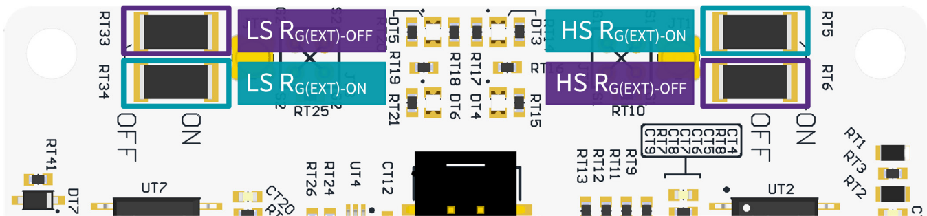
Figure 12: External turn-on and turn-off gate resistor locations
