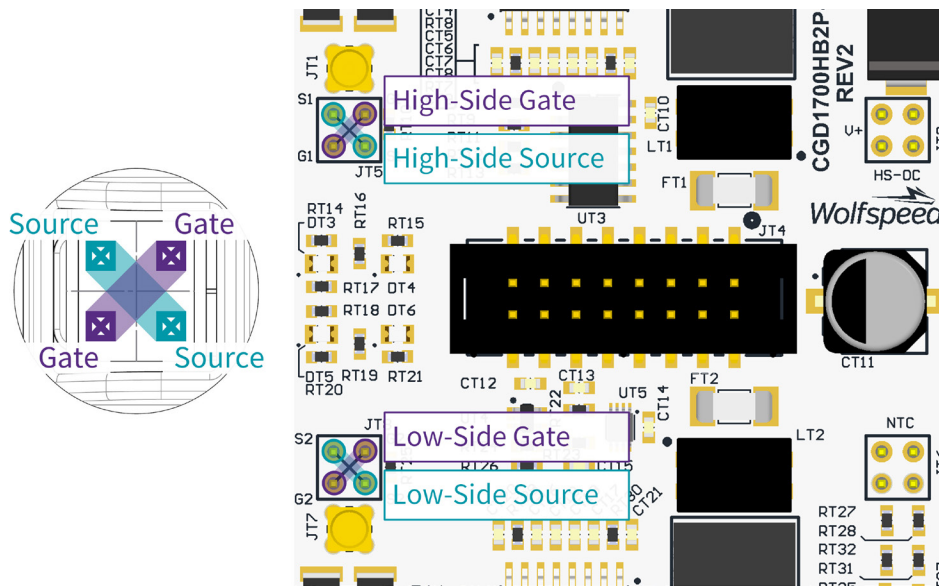
Figure 7: JT2 and JT5 output connectors orientations and pin locations
