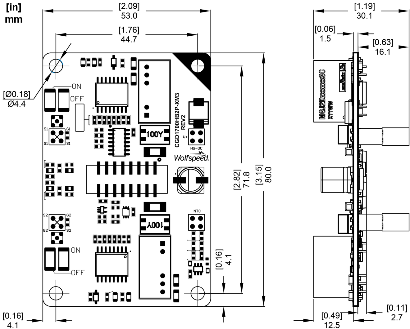
Figure 27: Dimensions of the CGD1700HB2P-XM3 gate driver
