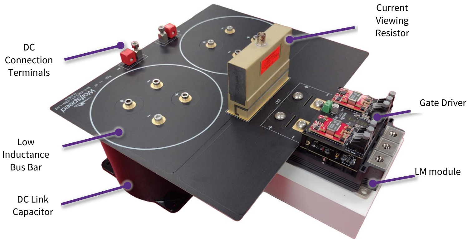
FIGURE 4: EVALUATION BOARD
