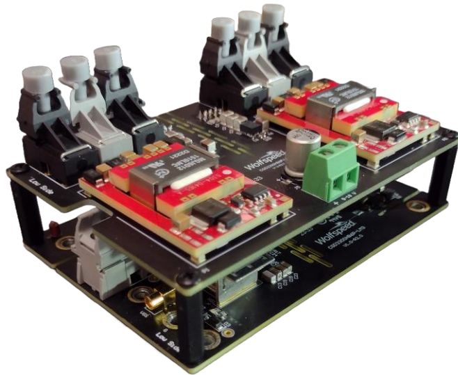
FIGURE 10: CGD1700HB2P-XM3 DUAL CHANNEL DIFFERENTIAL ISOLATED GATE DRIVER
