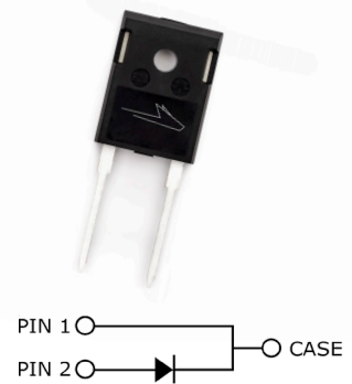
Package Types: TO-247-2 Marking: C4D20120H
