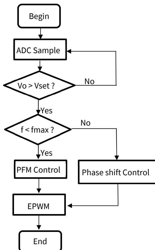
Figure 8: Flow chart of the control method in CRD22DD12N 22kW DC-DC converter
