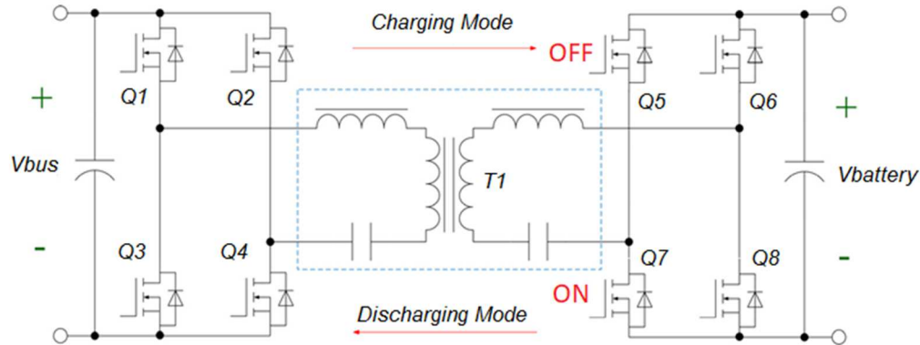
Figure 6: Half-bridge CLLC converter with full bridge SR in discharging mode
