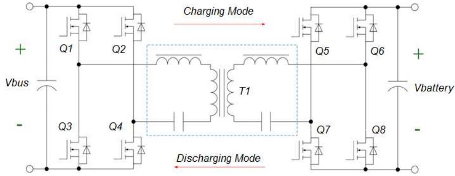
Figure 1: Schematic of a bi-directional DCDC converter
