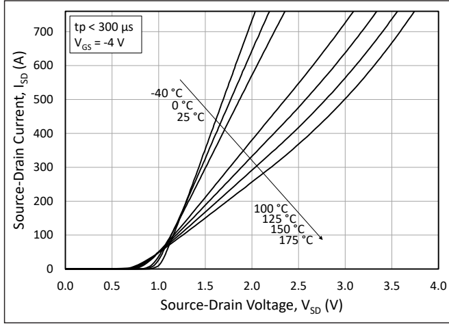
Figure 7. 3 rd Quadrant Characteristic vs. Junction Temperatures at V_{GS} = -4\text{ V}
