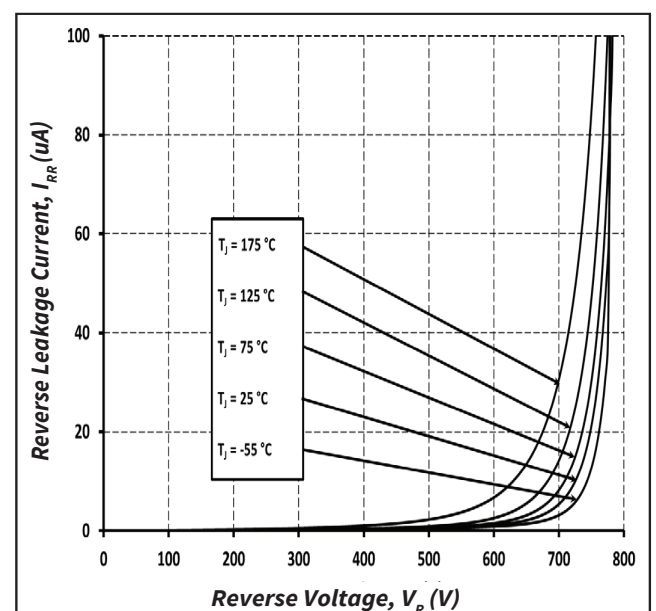
Figure 2. Reverse Characteristics
