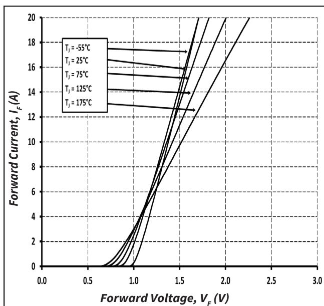
Figure 1. Forward Characteristics
