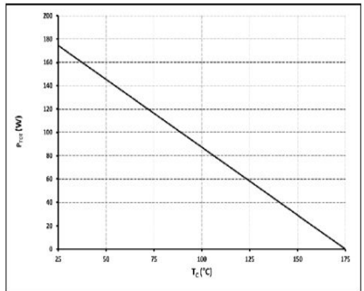
Figure 4 Power Derating
