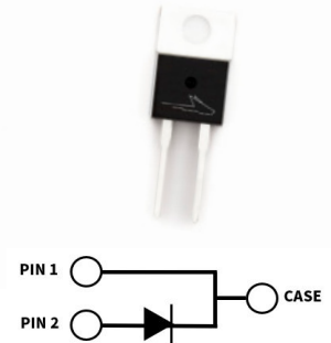
Package Types: TO-220-2 Marking: C6D20065A
