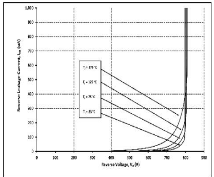
Figure 2 Reverse Characteristics
