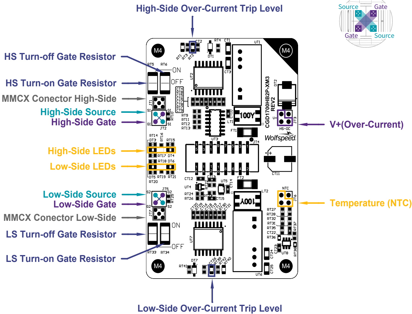
Gate Driver Interface
