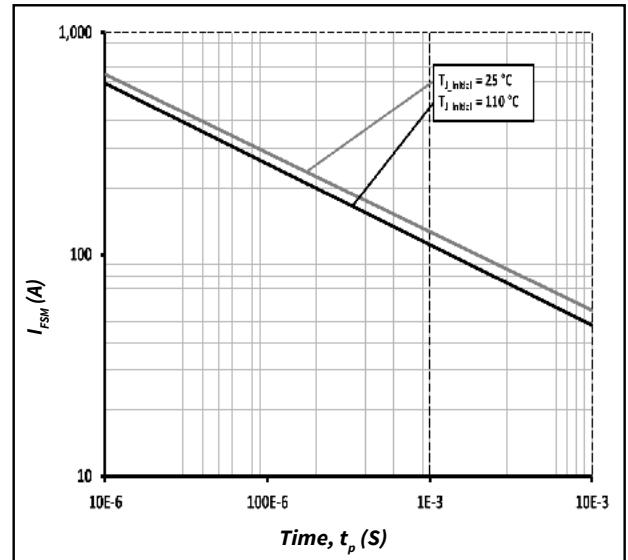
Figure 8. Non-Repetitive Peak Forward Surge Current (Sine Wave)
