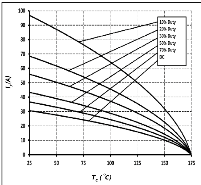
Figure 3. Current Derating
