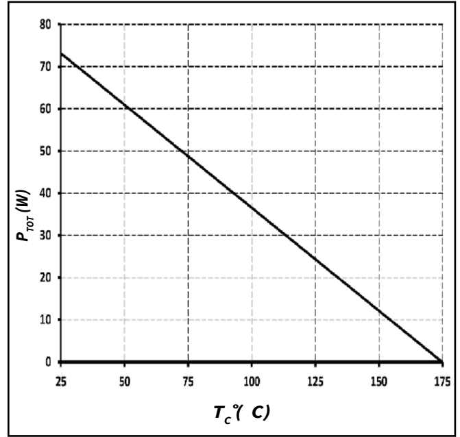
Figure 4. Power Derating
