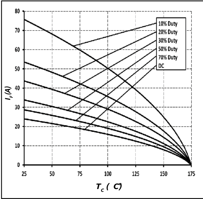
Figure 3. Current Derating
