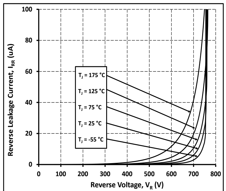
Figure 2. Reverse Characteristics
