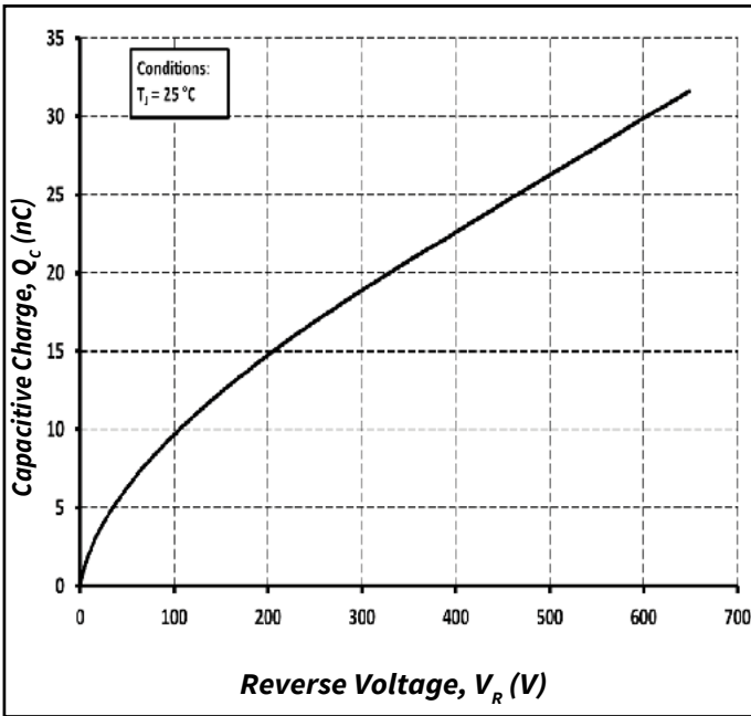
Figure 5. Total Capacitance Charge vs. Reverse Voltage
