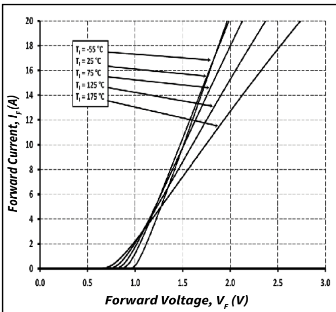
Figure 1. Forward Characteristics
