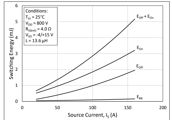
Figure 12. Switching Energy vs. Drain Current ( V_{DD} = 800 V)
