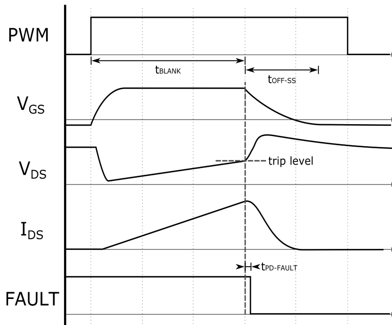
Over-Current Protection Timing Diagram
