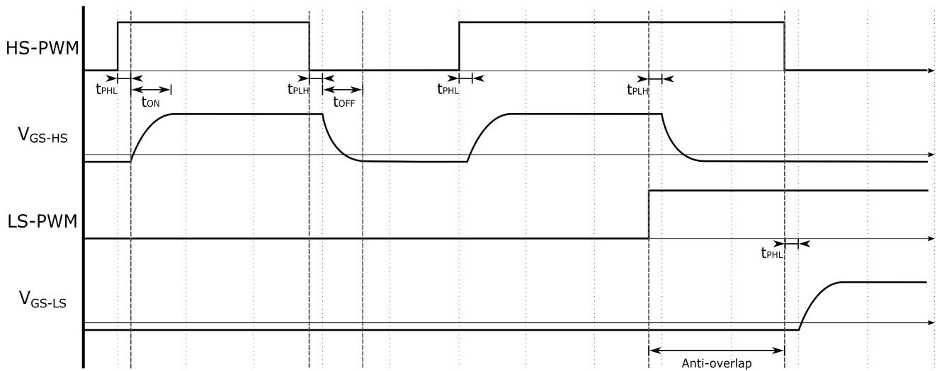
Gate Timing Diagram
