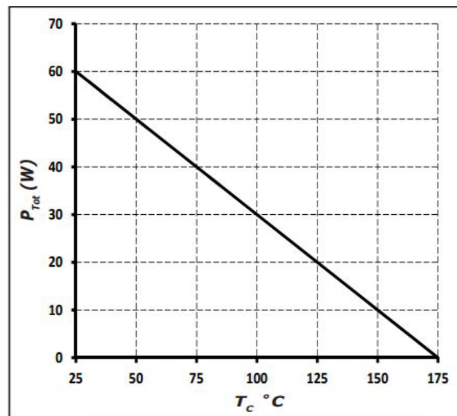
Figure 4 Power Derating
